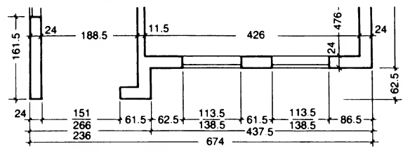
3 Dimensions of piers and apertures (drawn at 1:50 cm; units = cm)
